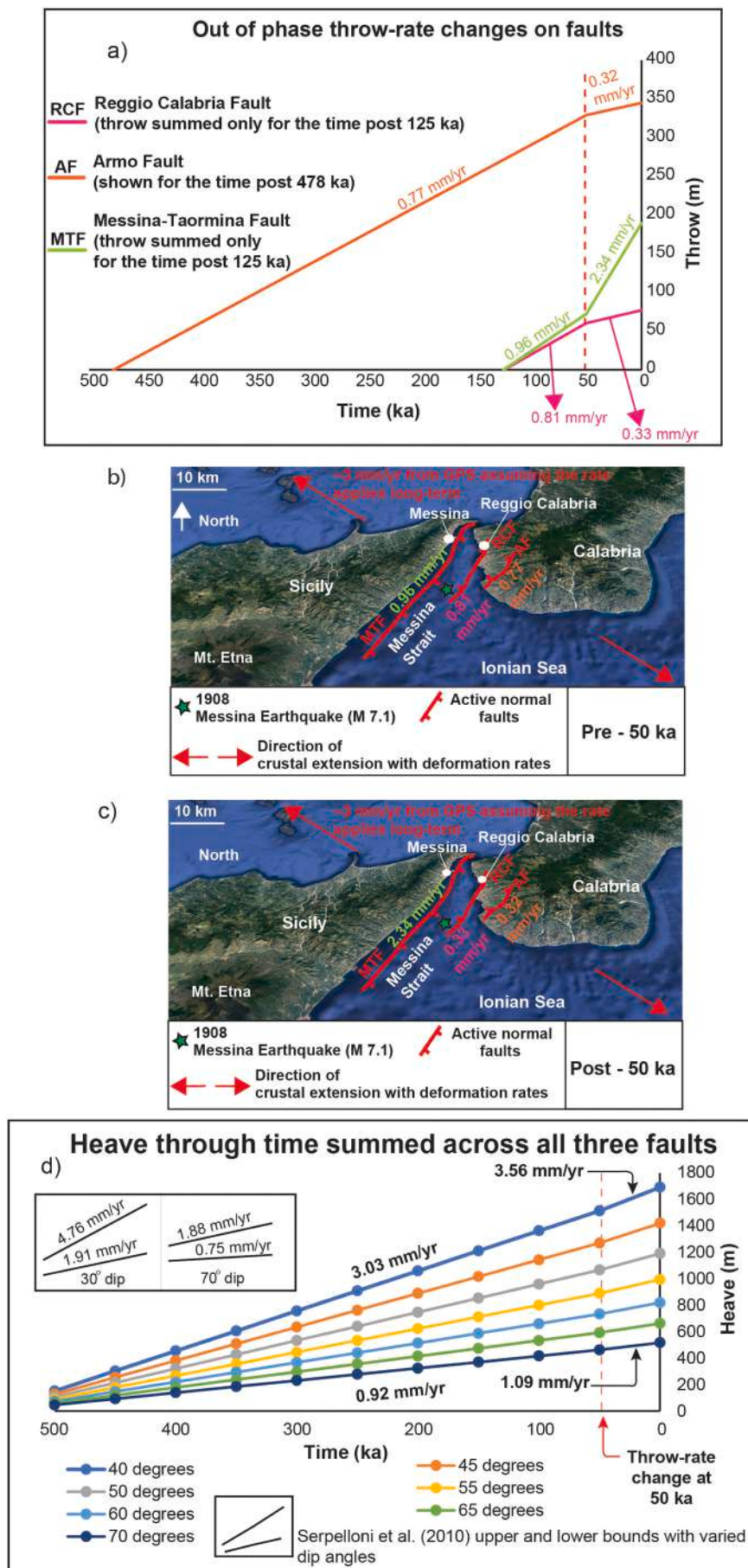
Fig. 10. (a) Throw-rates through time are shown for the Messina-Taormina Fault, Reggio Calabria Fault and Armo Fault. Changing throw rates through time have been calculated from faulted coeval marine terraces for the Reggio Calabria Fault and Armo Fault. In (b) and (c) a tectonic sketch with refined throw-rate through time, pre and post 50 ka, with horizontal extension rates from Serpelloni et al. (2010). Note that photos are from Google EarthTM (Maxar Technologies, Landsat). In (d), values of throw-rates-converted heave rates are shown, iterating different fault dip-angles for all 3 investigated faults, compared to those proposed by Serpelloni et al. (2010) using geodetic measurements. In (d), we assume that fault dip angles for all 3 investigated faults are the same because we have no information for those values. The contrast of changing throw-rates of individual faults with constant heave-rates when summed all the faults suggests that faults are interacting to maintain the regional extension rate.
