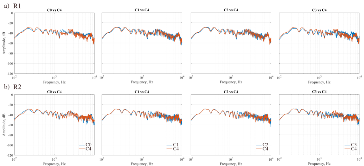
Figure 6. Measured impulse response spectral content results for C0, C1, C2, C3, and C4 configurations for both R1 and R2 positions (source in R2 and R1, respectively).
