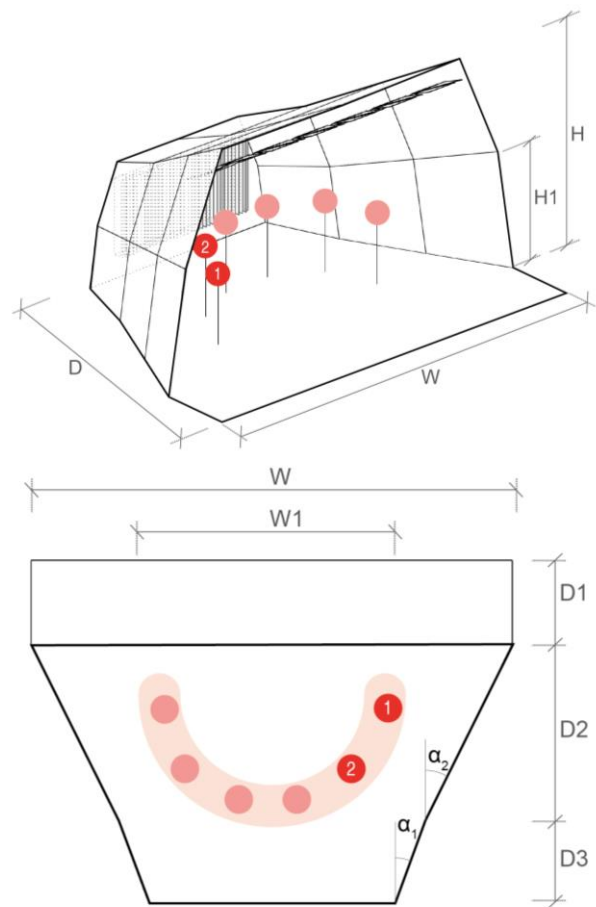
Figure 2. Main geometrical features of ReS: H=4.40\text{m} ; H_1=2.30\text{m} ; D=5.70\text{m} ; D_2+D_3=4.20\text{m} ; W=7.90\text{m} ; W_1=4.00\text{m} ; \alpha_1=20.4^\circ ; and \alpha_2=26.5^\circ .
