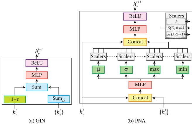
Fig. 1. Overview of GIN and PNA layers, where h_v^t and \{h_u^t\} denote the representation of, respectively, node v and its neighbors at layer t . GIN uses sum as the AGGREGATE function, followed by a sum and multi-layer perceptron (MLP) for the UPDATE function. PNA uses a set of aggregators (element-wise mean, standard deviation, maximum, and minimum) followed by degree-scalers (identity, amplifier, and dampener) as the AGGREGATE function. The UPDATE function consists of a concatenation followed by an MLP.
