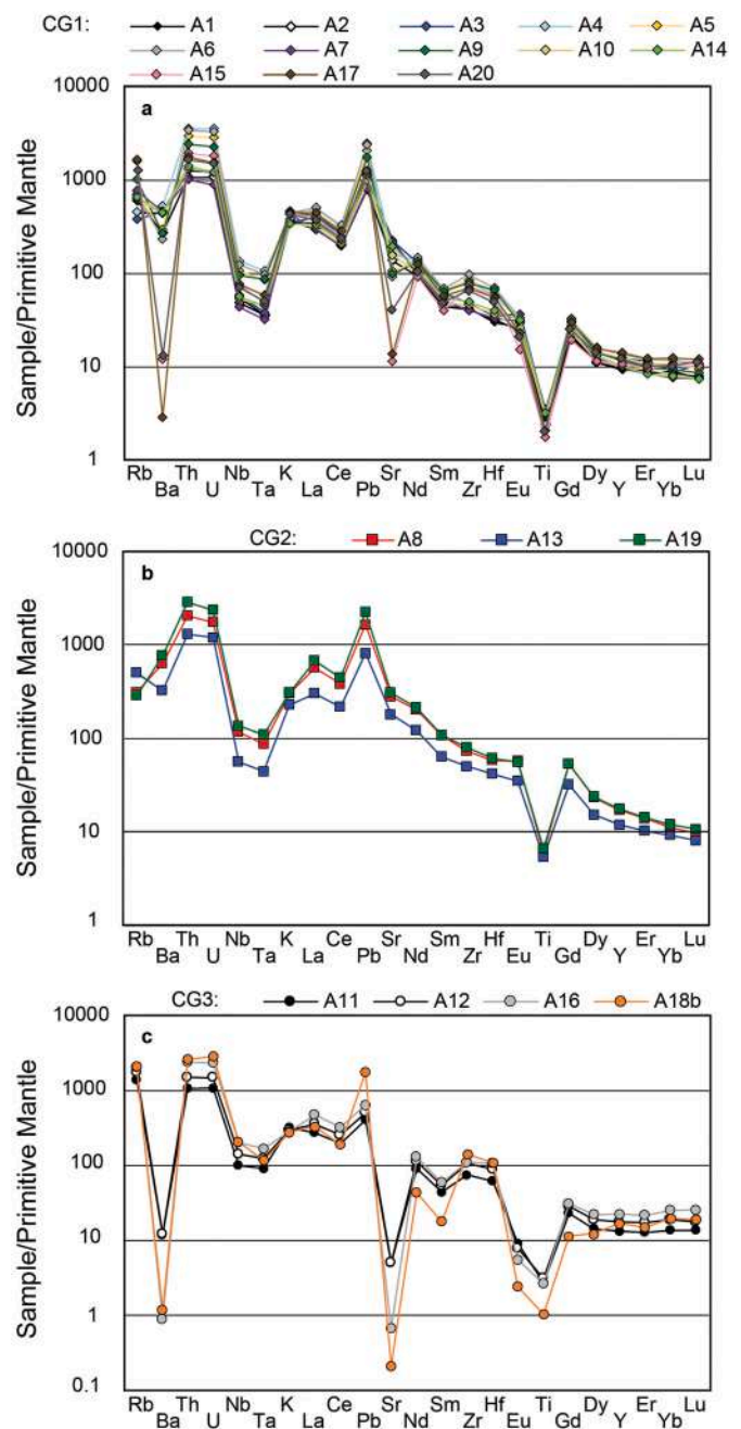
Fig. 4. Primitive mantle normalized trace elements distribution of the Acerno tephra layers (normalization values from Lyubetskaya and Korenaga, 2007).
