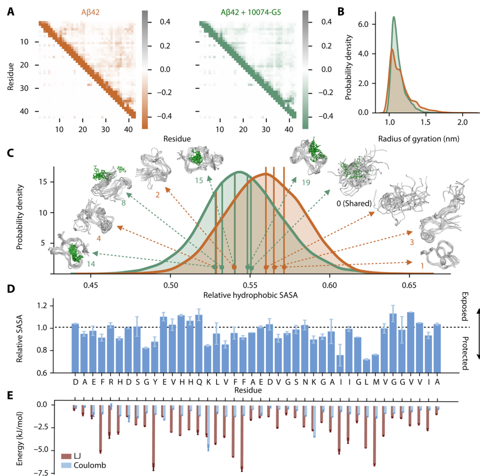
Fig. 2. Metadynamic meta-inference simulations characterize the dynamic binding and show how 10074-G5 promotes A \beta 42 conformations with less hydrophobicity. (A) Metadynamics meta-inference simulations demonstrate that inter-residue contact maps for Lennard-Jones (LJ) (top right) and Coulomb (top left) potentials for the unbound (orange) and the bound (green) structural ensembles of A \beta 42 with 10074-G5 are highly similar. (B) Radii of gyration for the unbound and bound structural ensembles are also highly similar (shown using kernel density estimates of A \beta 42 with 10074-G5 are shown using kernel density estimates of A \beta 42 with 10074-G5 are shown using kernel density estimates based on metadynamics weights using a Gaussian kernel). (C) Relative hydrophobic solvent accessible surface area (SASA) of A \beta 42 (total hydrophobic area over total surface area) of the bound and unbound ensembles, showing that 10074-G5 decreases the relative exposed hydrophobicity of A \beta 42. The holo ensemble was calculated only on the protein surface but accounts for the presence of the compound. Data are shown using kernel density estimates as described in (B). Some of the representative structures from these distributions are shown. Numbers indicate cluster IDs shown in Fig. 3. (D) Ratio (bound/unbound) of the ensemble-averaged, total SASA per residue showing regions of A \beta 42 that become more exposed or protected in the presence of 10074-G5. SASAs of the bound ensemble were calculated on the protein in the presence of 10074-G5. (E) Ensemble-averaged, residue-specific LJ and Coulomb interaction energies show that 10074-G5 has strong interactions with aromatic and charged residues. Error bars represent SDs between first and second halves of the analyzed trajectories in (D) and (E).
