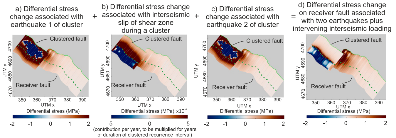
Fig. 3. Modelling approach for deriving the differential stress change imparted on a receiver fault due to earthquake clustering occurring on a neighbouring fault/shear-zone. Solid green line is the fault surface trace. Dashed green line is the limit between brittle fault and viscous shear-zone. Each plot is obtained with Coulomb 3.4 (Toda et al., 2005).
