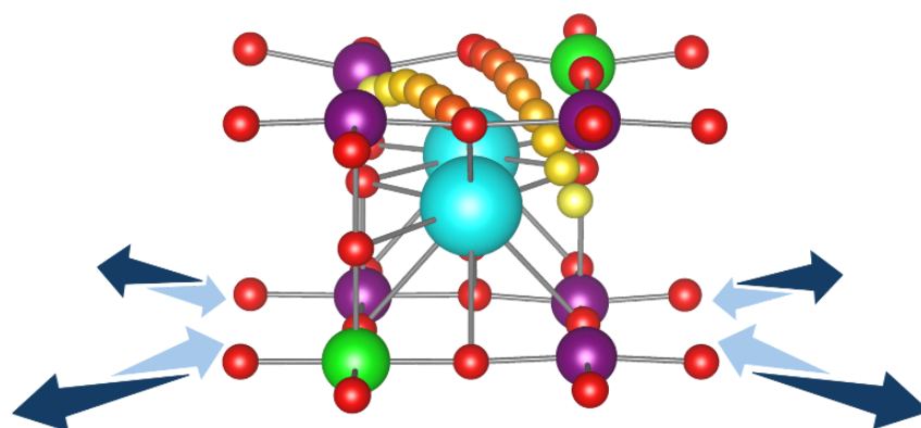
Figure 1: Pictorial representation of V_{\text{O}} -mediated migration in \text{Sr}_2\text{Fe}_{1.5}\text{Mo}_{0.5}\text{O}_{6-\delta}
