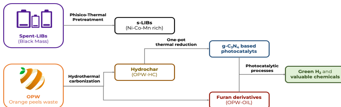
Scheme 1. Development of low-cost and robust heterogeneous photocatalysts starting from spent-Li ion batteries (s-LIBs) and orange peel waste (OPW) and in their application in the sustainable production of green H 2 and added value chemicals
