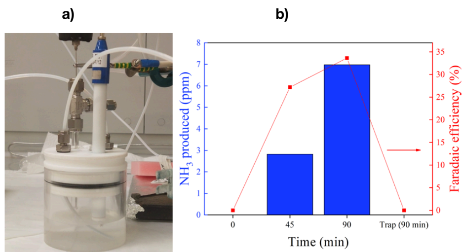
Figure 1: a) Plasma-Liquid electrochemical cell and b) yield to ammonia (ppm) and corresponding Faradaic efficiency (%) at 2 mA after 45 and 90 minutes.
