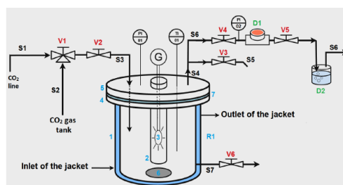
Figure 1: Demonstration of the structure of the high pressure photoreactor.
