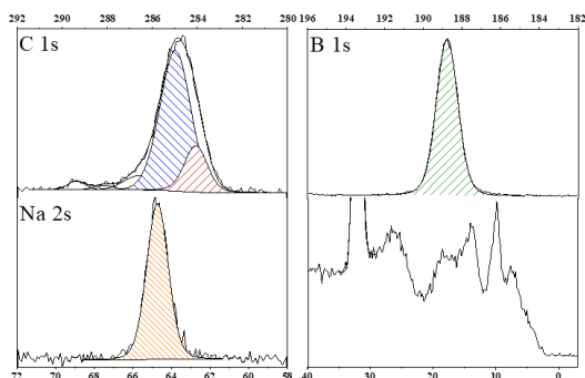
Figure 1: C 1s, B 1s, Na 2s and valence XPS spectra of the pristine compound.
