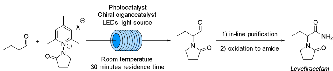
Figure 1: Continuous flow telescoped process for the synthesis of Levetiracetam
