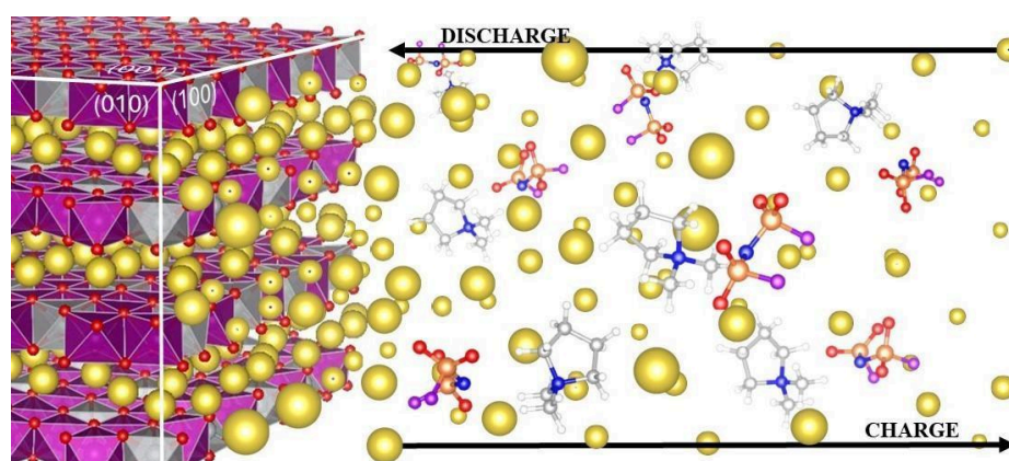
Figure 1 Pictorial representation of P2- \text{Na}_x\text{Ni}_{0.25}\text{Mn}_{0.75}\text{O}_2 /PyrFSI interfaces
