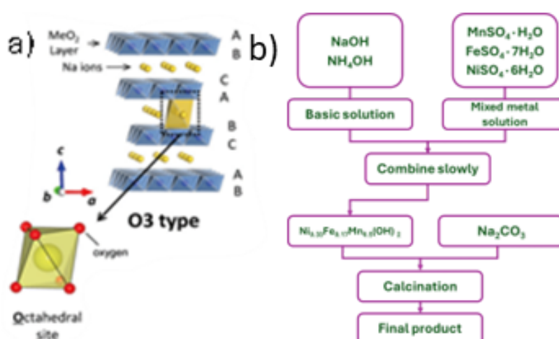
Figure 1: a) O3-type structure; b) synthesis protocol.
