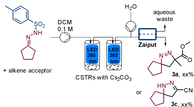
Figure 1: Photo-CSTR cascade with integrated in-line work up using Zaiput membrane technology.
