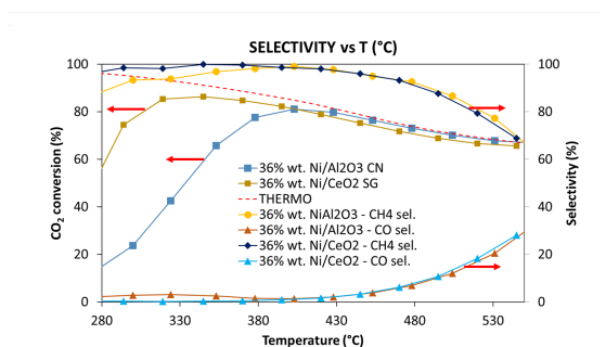
Figure 1: CO 2 conversion and selectivity as function of T
