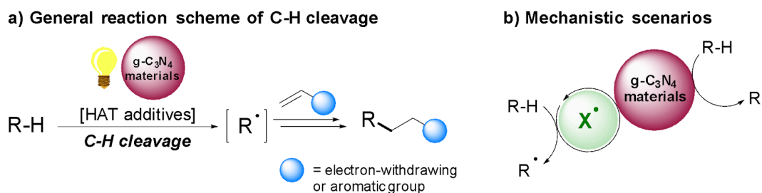
Figure 1: Carbon nitride materials as heterogeneous photocatalyst in C–H bonds functionalization: i) General reaction scheme; ii) Mechanistic scenarios.
