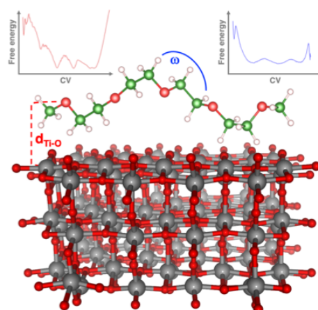
Figure 1: Configurational and conformational structuring at (101)-TiO 2 /PEO interfaces.
