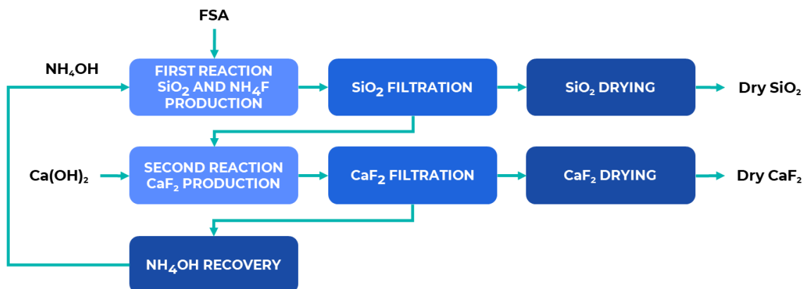
Figure 1: LIFE-SYNFLUOR process flow diagram.
