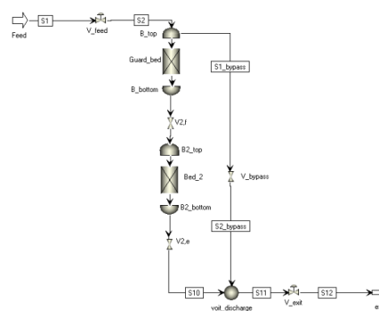
Figure 1: Simulated flowsheet for GHGs capture. Aspen Adsorption ® V11.
