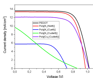
Figure 1: J-V curves of DSSCs based on PEDOT and organometallic polymers.
