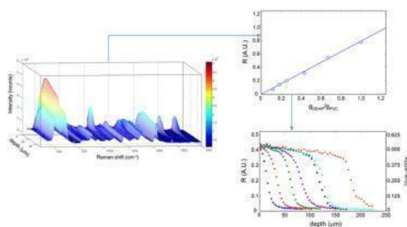
Figure 1: Migration results after 2 days: Raman spectra of rPVC film in contact with pPVC@DEHP; DEHP calibration curve; CRM profiles for DEHP migration from pPVC@DEHP.
