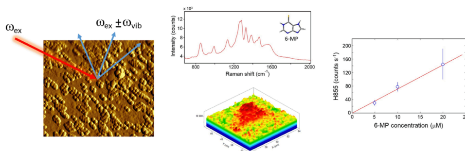
Figure 1: AFM image of 2D platform; SERS spectrum of 6-MP; AFM/Raman map of 6-MP; calibration curve for the quantitative analysis of 6-MP.
