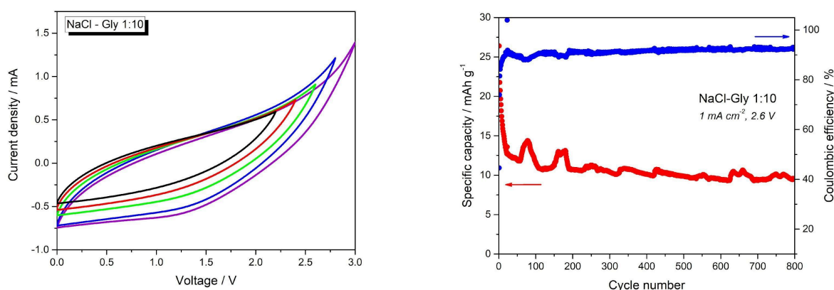
Figure 1: Electrochemical test of NaCl-Gly 1:10 in EDLC
