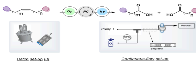
Figure 1: Batch and flow set-up in the oxidative cleavage of unsaturated fatty acids.
