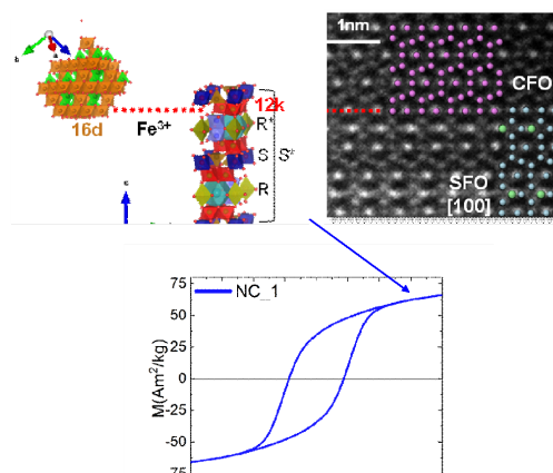
Figure 1: High-resolution HAADF-STEM image of a typical SFO/CFO interface in NC_1 and corresponding magnetic hysteresis loop at 300K.
