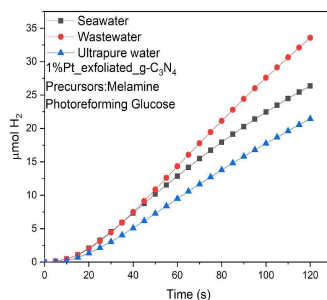
Figure 1: Photocatalytic H 2 production by immobilized Pt/g-C 3 N 4 (powder) using different water sources.
