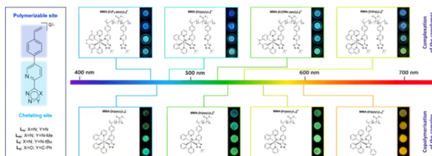
Figure 1: General structure of the polymerizable ligands; materials structures and appearance under UV light.
