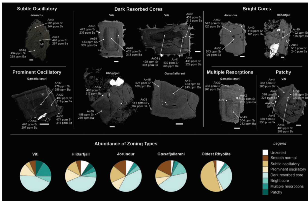
Fig. 5. Labeled back-scattered electron (BSE) images of selected plagioclase crystals, highlighting zoning types and associated variations in An, Sr, and Ba content. Pie charts show the relative proportion of each zoning type within each unit. Melt inclusions are labelled 'MI'. Scale bars are 100 \mu\text{m} .
