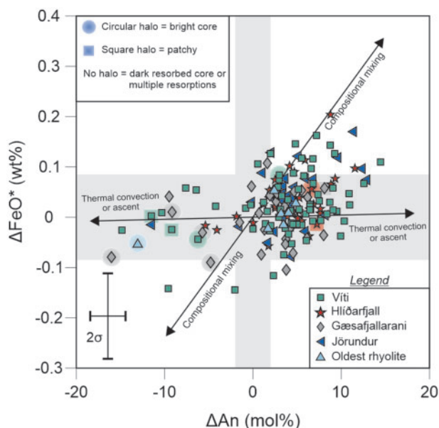
Fig. 12. Compositional changes across plagioclase internal resorption surfaces. \Delta\text{An} = change in plagioclase An (mol%; outer zone—inner zone). \Delta\text{FeO}^* = change in total Fe expressed as FeO (wt%; outer zone—inner zone). Compositional mixing and thermal convection or ascent vectors after Ruprecht & Wörner (2007). Compositional changes plotting within the grey fields are less than the 2\sigma analytical uncertainty.
