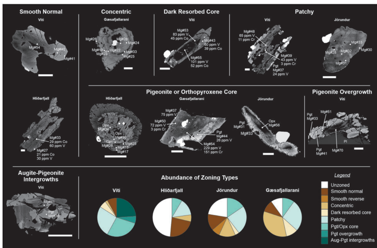
Fig. 7. Labelled BSE images of selected augite crystals ( \pm pigeonite and/or orthopyroxene), highlighting different zoning types. Pie charts show the relative proportion of each zoning type within each unit. All analyses are augite unless specified: Pgt = pigeonite; Opx = orthopyroxene; Pl = plagioclase. Scale bars are 100 \mu m.
