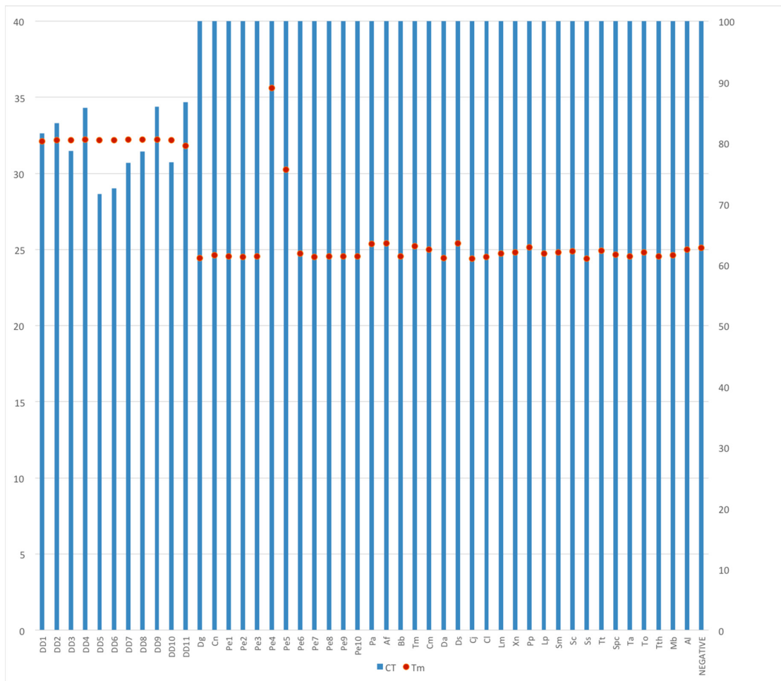
Figure 4. Real-time PCR. Threshold cycles (Ct) on the left and melting temperature (Tm) on the right. Abbreviations as in Tables 1 and 2.
