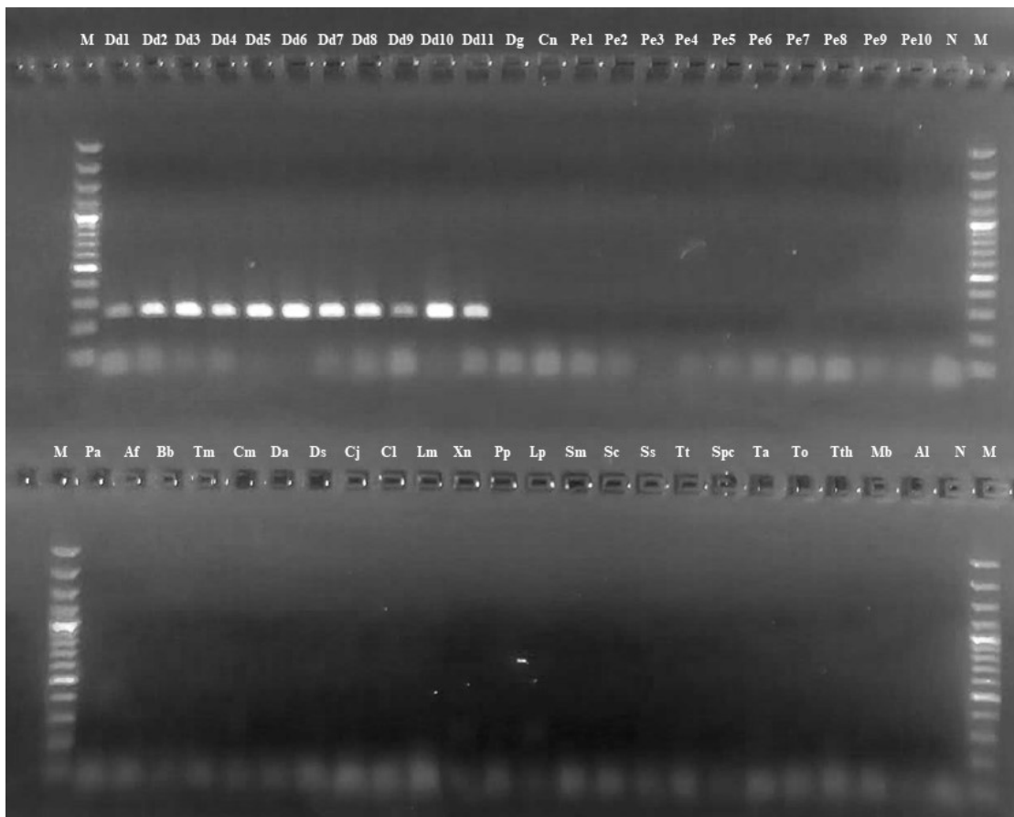
Figure 3. Gel electrophoretic image. End-point PCR amplification of the NAD2 fragment in the 11 D. dentex specimens considered in this study (lanes 2–12, from Dd1 to Dd11). No amplification was obtained for all the other fish species (lanes 13–24 and 25–47). Abbreviations as in Tables 1 and 2. N: negative control; M: 100 bp ladder.
