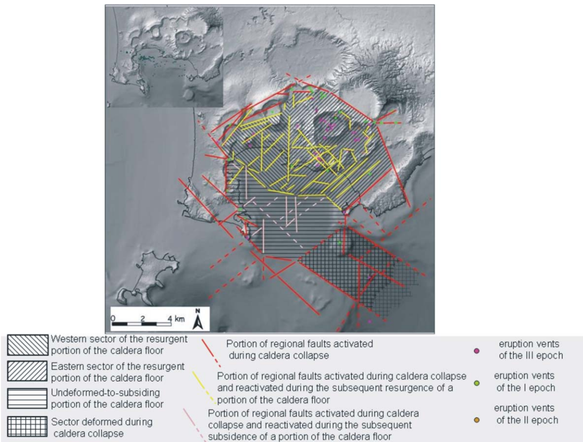
Figure 6. Structural sketch map of the Neapolitan Yellow Tuff caldera. The inset shows the distribution of the fumaroles; the offshore ones are from De Bonitatibus et al. [1970].
