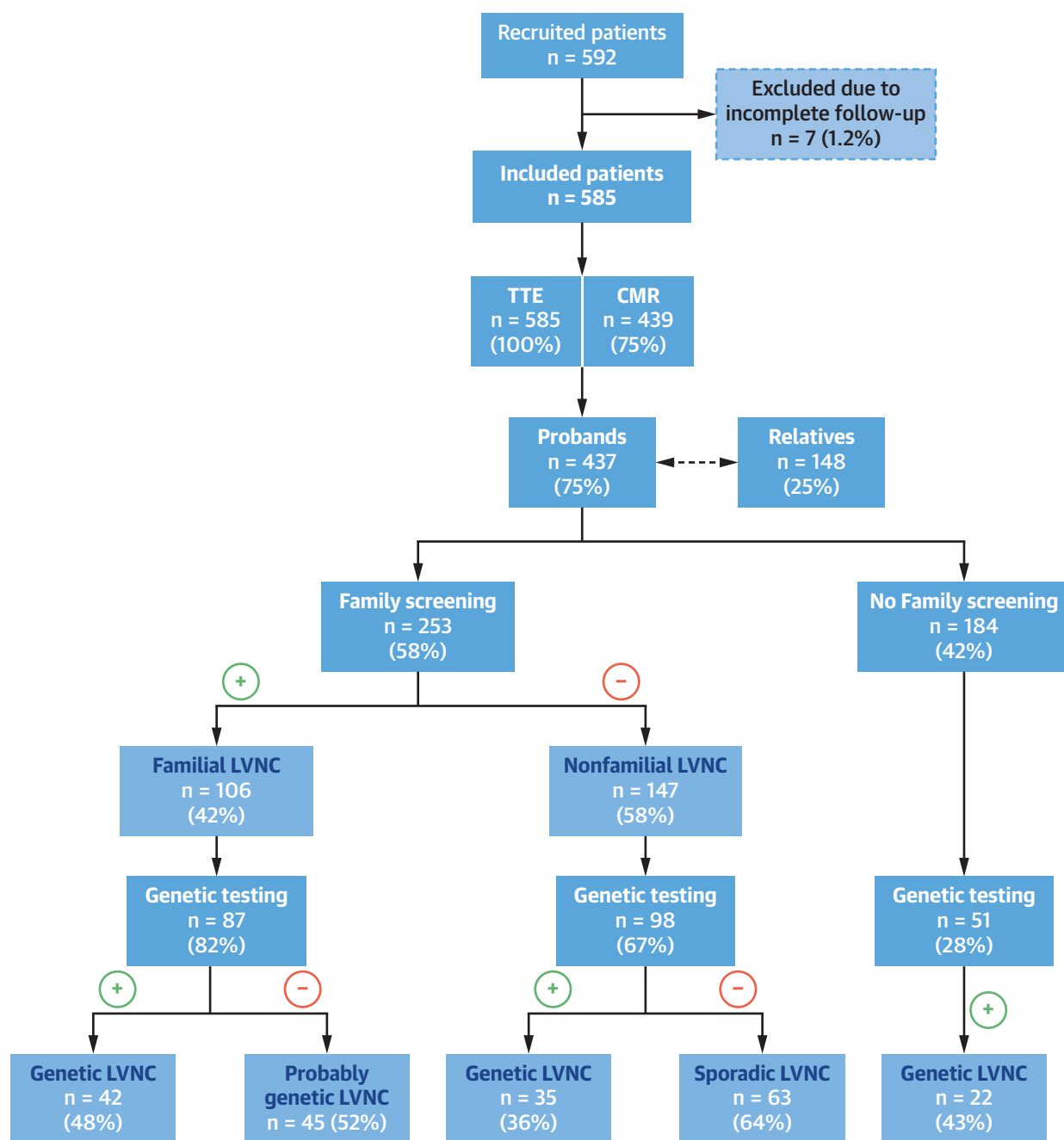
FIGURE 1 Study Flowchart
