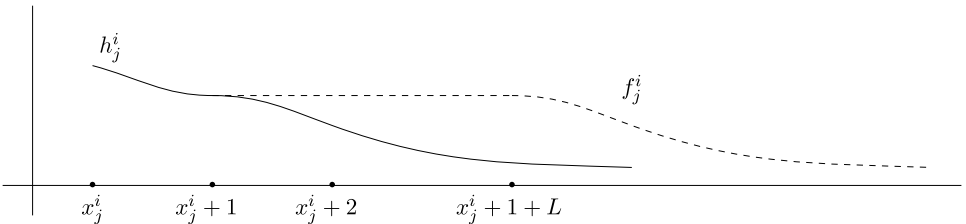
Fig. 1. Qualitative picture of the functions h_j^i and f_j^i .
