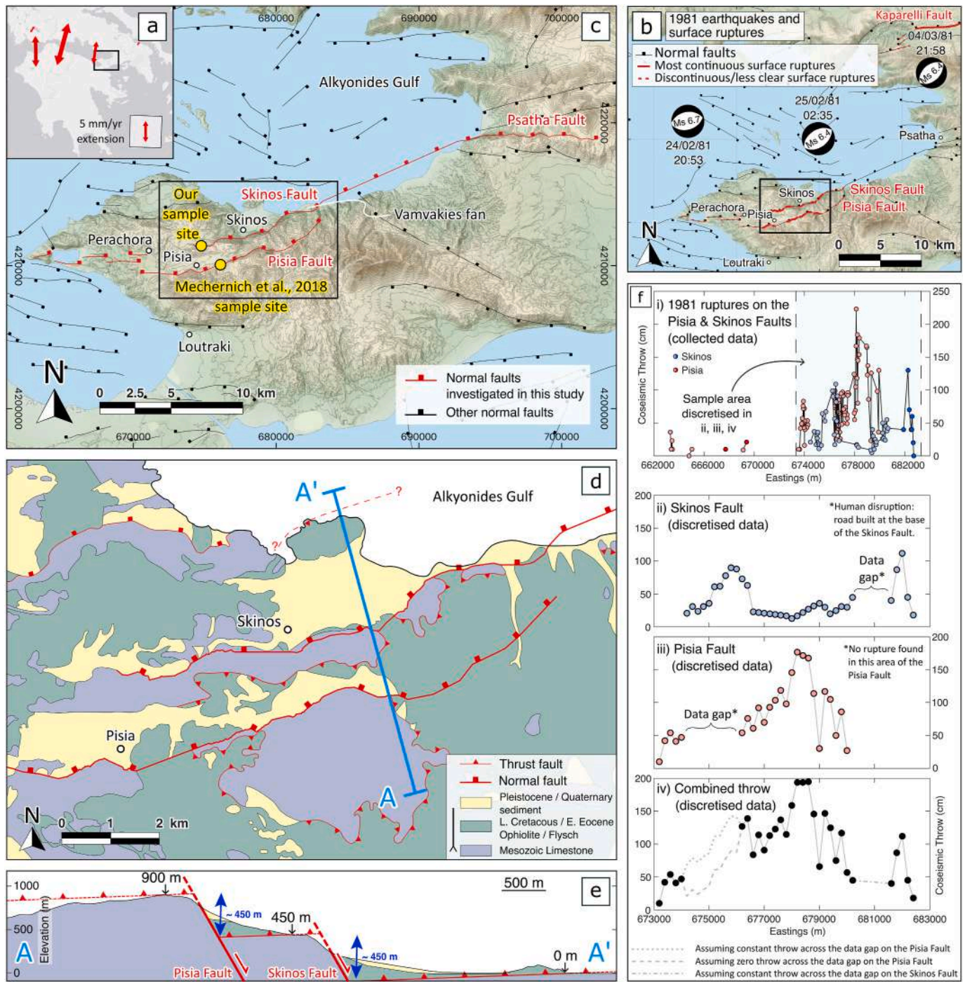
Fig. 1. Details of the Pisia and Skinos Faults. (a) Coastline map of mainland Greece with extension rates from Briole et al. (2021) and the location of area (c) in the black box. (b) Map of the 1981 surface ruptures (red solid) on the Pisia, Skinos and Kaparelli Faults (Jackson et al., 1982; Mitchell et al., 2024) and the location of the ruptures in (f.ii,iii,iv) in the black box. Focal mechanisms are displayed at the inferred epicentres of the three earthquakes of the 1981 eastern Gulf of Corinth earthquake sequence (Hubert et al., 1996). (c) Map of the Perachora Peninsula and the eastern Gulf of Corinth region with surface traces of normal faults (Ganas et al., 2013; Mitchell et al., 2024) showing the entire South Alkyonides Fault System (Pisia, Skinos and Psatha Faults) and the location of area (d) in the black box. The locations of the ^{36}\text{Cl} sample sites are shown in yellow. The Skinos Fault sample site is located at 674762 m E, 4211384 m N (lat 38.033325°, long 22.991320°) and the Pisia Fault sample site (Mechernich et al., 2018) is located at 676105 m E, 4210067 m N (lat 38.021202°, long 23.006291°). (d) Geological map of the area of overlap between the across-strike Skinos and Pisia Faults with a cross-section line for (e) oriented NNW-SSE using map sheets (1:50,000) Kaparellion and Perachora (IGME Kaparellion Geological Map Bornovas et al., 1984; IGME Perachora Geological Map Bornovas et al., 1984). (e) Cross-section through the Pisia and Skinos Faults showing the offset of a thrust of ~450 m each (lithology key is the same as in (d)). (f) Comparing the 1981 coseismic throw profiles on the Pisia and Skinos Faults (data sourced from Mitchell et al., 2024 with additional measurements from Collier et al., 1998; Roberts and Ganas, 2000). (i) Field measured coseismic throw data from the Perachora Peninsula to Vamvakies Fan. Pale and dark blue circles are Skinos Fault data recorded by Mitchell et al. (2024) and Collier et al. (1998) respectively. Pale and dark red circles are Pisia Fault data recorded by Mitchell et al. (2024) and Roberts and Ganas (2000) respectively. Solid line connects data of ruptures on each fault. In (ii) and (iii) the throw profiles of the Skinos and Pisia Faults are discretised from the data in (i), respectively. (iv) Combined discretised data by summing the throw values from (ii) and (iii). Coordinate system: WGS 84/UTM Zone 34 S. (For interpretation of the references to colour in this figure legend, the reader is referred to the Web version of this article.)
