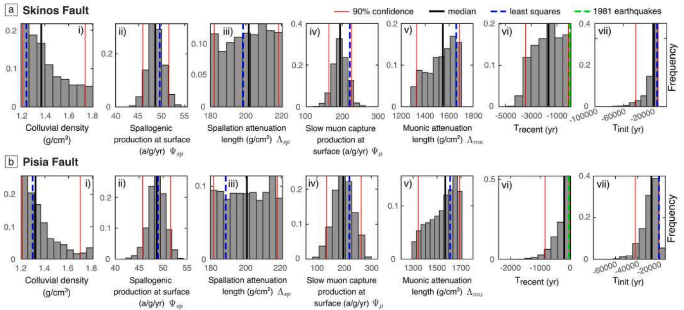
Fig. 6. Parameters iterated in the MCMC modelling of the ^{36}\text{Cl} data on the (a) Skinos Fault and (b) Pisia Fault. Medians and 90 % confidence from the posterior distributions after 50 % burn-in for (i) colluvial density, (ii) spallogenic production, (iii) spallation attenuation length, (iv) slow muon capture, (v) muonic attenuation length, (vi) age of last earthquake ( T_{\text{recent}} ) and (vii) age from which production is preserved ( T_{\text{init}} ), and the values for the least squares solution. The 1981 earthquakes are indicated on (vi).
