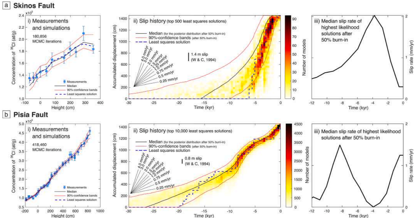
Fig. 4. Measured ^{36}\text{Cl} concentrations and slip histories recovered by modelling for the (a) Skinos Fault ( ^{36}\text{Cl} concentrations from our study) and (b) Pisia Fault ( ^{36}\text{Cl} concentrations from Mechernich et al., 2018 and remodelled herein). (a.i,b.i) Measured ^{36}\text{Cl} concentrations versus distance in the plane of the fault for the samples extracted at the sites in Fig. 3 with the modelled replications of the data from MCMC modelling of the ^{36}\text{Cl} data. (a.ii,b.ii) Slip histories recovered from the modelling. The word “top” refers to the solutions which minimise the sum of the residuals between measured and modelled ^{36}\text{Cl} concentrations. (a.iii,b.iii) Median slip rates for the same model runs as (a.ii) and (b.ii) after 50% burn-in. The median slip rate is calculated by size of slip events multiplied by their frequency divided by bin size for all model runs in the posterior distribution and bin size is defined as the optimal bin size for the distributions. See Beck et al. (2018) and Roberts et al. (2024) for more details of the modelling procedure and methods for displaying results.
