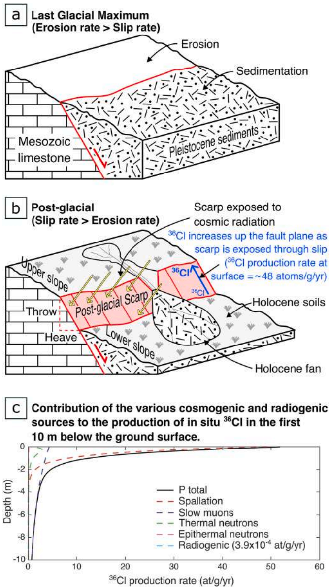
Fig. 2. Evolution of post-glacial scarps and the production of ^{36}\text{Cl} on fault planes due to exposure through slip. Illustration (a) demonstrates no fault scarp preservation above the surface during the last glacial maximum (adapted from Roberts and Michetti, 2004); (b) demonstrates fault scarp preservation above the surface during/after the demise of the last glacial maximum (adapted from Roberts and Michetti, 2004). Graph (c) shows the contribution of the various cosmogenic and radiogenic sources to the production of in situ ^{36}\text{Cl} in the first 10 m below the ground surface (modified from Schlagenhauf et al., 2010).
