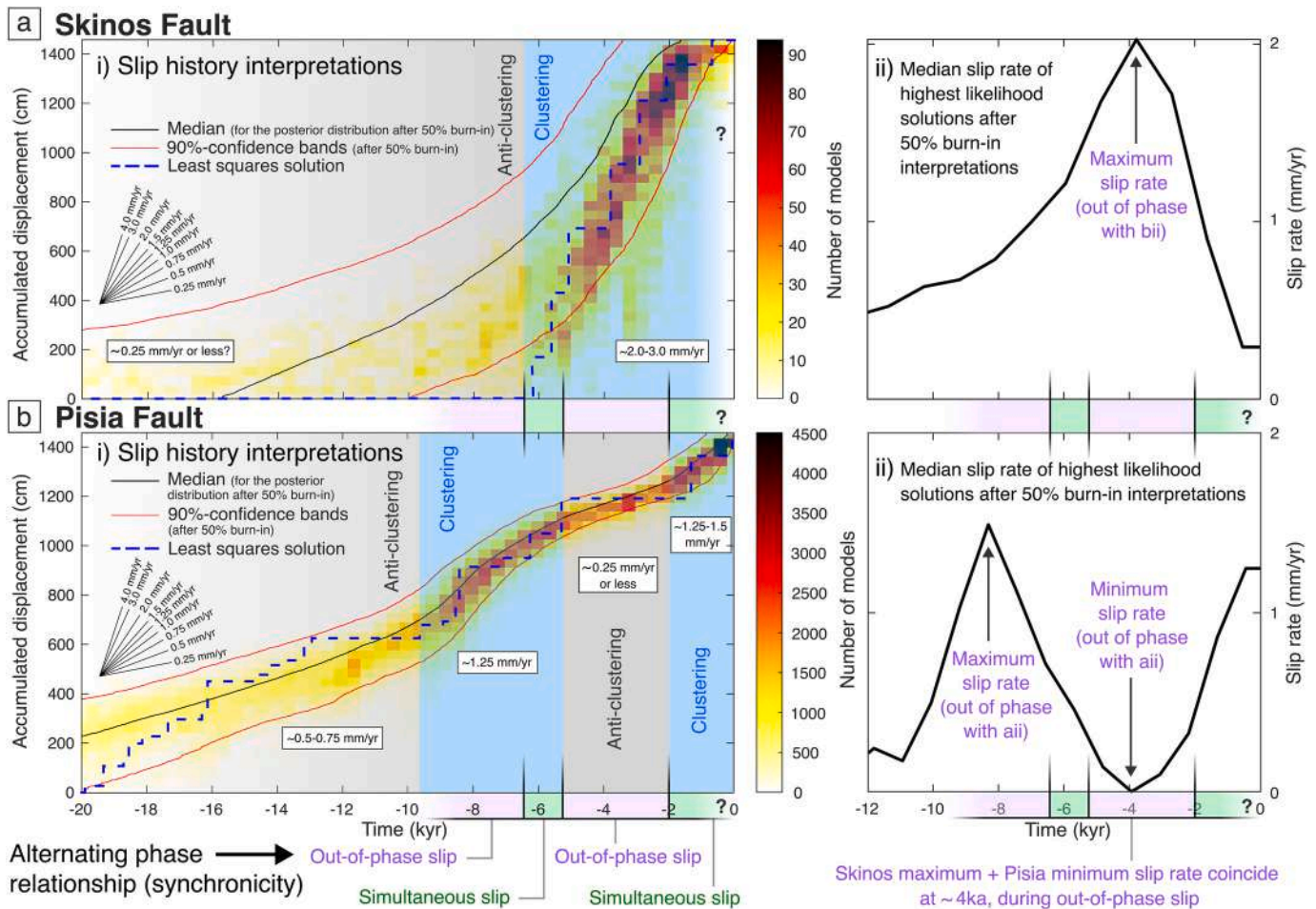
Fig. 5. Interpretations of slip histories for the (a) Skinos Fault and (b) Pisia Fault. (a.i,b.i) Slip in the planes of the faults indicated by the least squares solutions, the ensemble of least squares solutions and the posterior distribution derived from MCMC modelling of the ^{36}\text{Cl} data. The interpreted slip rates in white boxes are averaged within each period. Blue rectangles show periods of high slip rate (temporal cluster). Grey rectangles show periods of relatively low slip rate (temporal anticluster). Purple rectangles indicate periods when one fault is experiencing a high slip rate while the other is in a low slip rate. Green rectangles indicate periods when both faults are experiencing relatively high slip rates. (a.ii,b.ii) Out-of-phase slip behaviour indicated by the median slip rate of highest likelihood solutions derived solely from the posterior distribution after 50% model burn-in for the same model runs as (a.i) and (b.i). (For interpretation of the references to colour in this figure legend, the reader is referred to the Web version of this article.)
