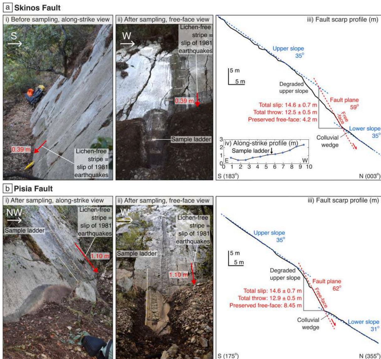
Fig. 3. ^{36}\text{Cl} sample sites and fault scarp field measurements on the (a) Skinos Fault and (b) Pisia Fault (see Mechernich et al., 2018 , their sample site P6). (a.i,b.i) Limestone fault plane site photographs of (a) the Skinos Fault before sampling, and of (b) the Pisia Fault after sampling with an along-strike view. (a.ii,b.ii) Site photographs of the sample ladder on the fault planes and clear lichen-free stripes of the 1981 earthquake rupture with the view facing the free-face. (a.iii,b.iii) Topographic scarp profiles parallel to the slip vectors recorded in (a) the study herein and (b) Mechernich et al. (2018) . (a.iv) Along-strike profile of the hanging wall cut-off. Note the preserved freeface is larger at the Pisia site than the Skinos site.
