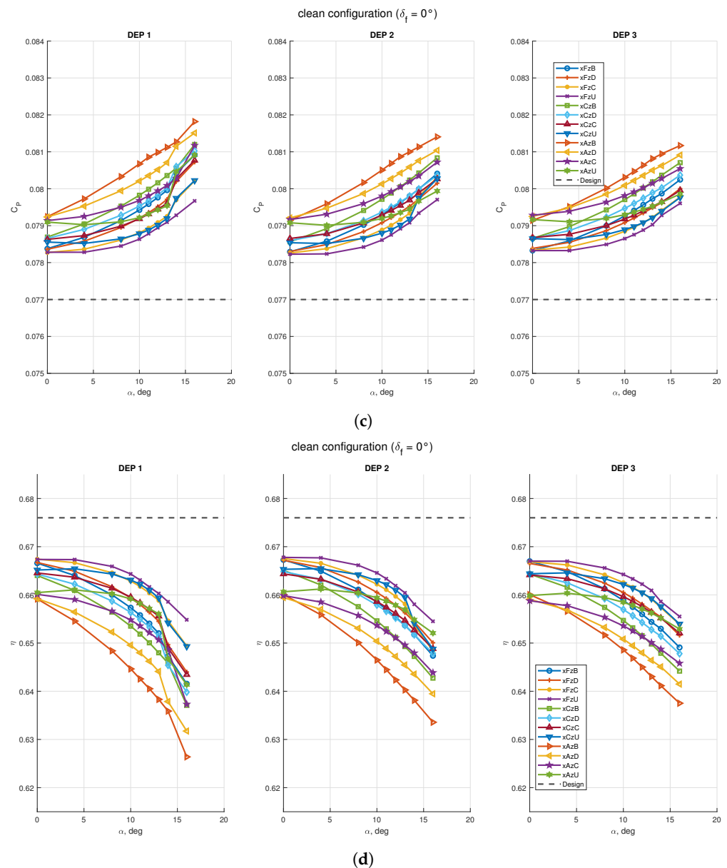
Figure 16. Effects of the wing on propeller performance with STAR-CCM+ virtual disk model: (a) propellers advance ratio; (b) propellers' thrust coefficient; (c) propellers' power coefficient; (d) propellers' efficiency. Design data is taken from Table 6, which are the assigned coefficients for the isolated propeller.
