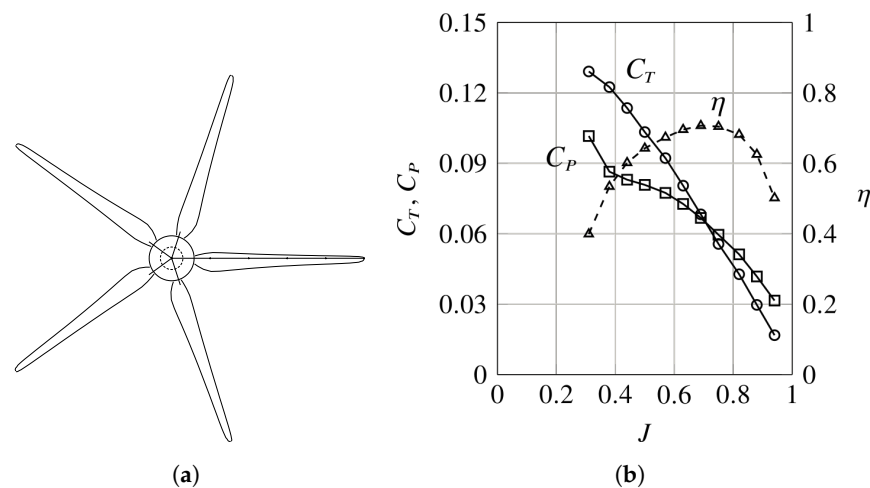
Figure 9. High-lift propeller designed with XROTOR: (a) propeller planform; (b) propeller characteristics.
