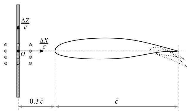
Figure 2. Positions of the propellers' array. The black circle is the baseline location.
