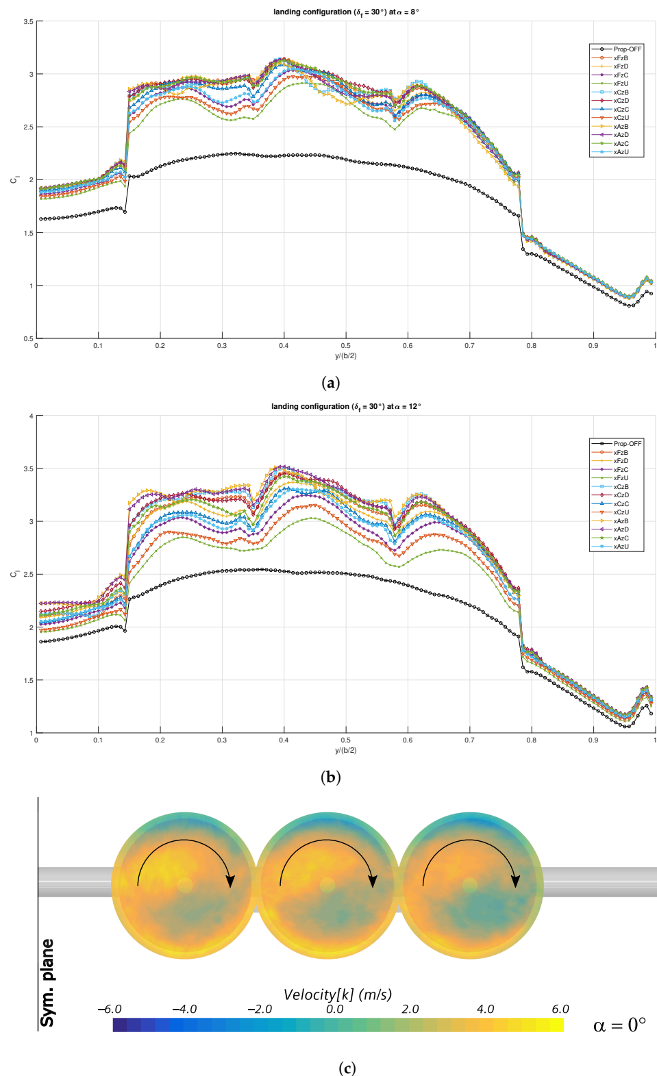
Figure 27. Spanwise section lift distributions for the wing with flap deflected for landing: (a) \alpha = 8^\circ ; (b) \alpha = 12^\circ ; (c) vertical velocity component in the disk plane.
