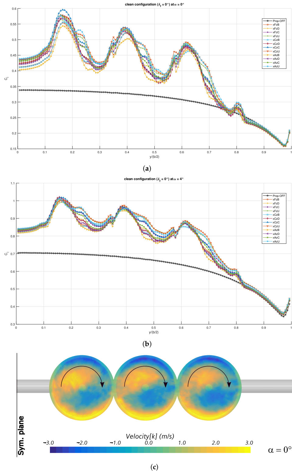
Figure 13. Spanwise section lift distributions for the clean wing: (a) \alpha = 0^\circ ; (b) \alpha = 4^\circ ; (c) vertical velocity component in the disk plane.
