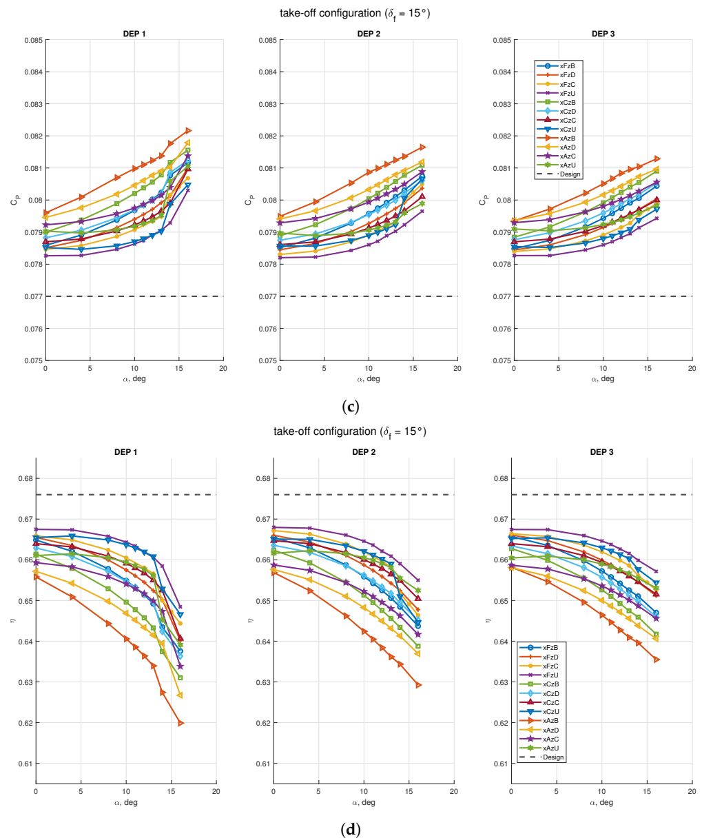
Figure 23. Effects of the wing with flap deflected for take-off on propellers' performance with STAR-CCM+ virtual disk model: (a) propellers' advance ratio; (b) propellers' thrust coefficient; (c) propellers power coefficient; (d) propellers' efficiency. Design data are taken from Table 6, which are the assigned coefficients for the isolated propeller.
