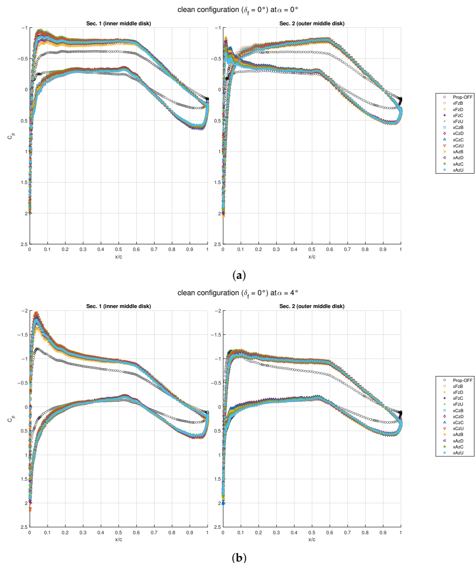
Figure 14. Chordwise pressure distributions for the clean wing around the mid propeller: (a) \alpha = 0^\circ ; (b) \alpha = 4^\circ .
