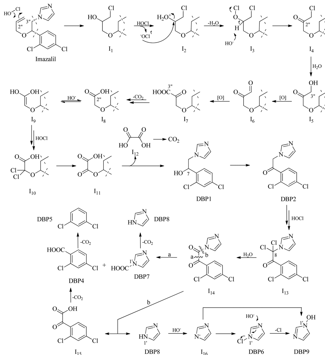
Fig. 2 Proposed reaction mechanism leading to the formation of DBP1-DBP2 and DBP4-DBP9. The lowercase letters in the figure indicate different reaction mechanisms.
