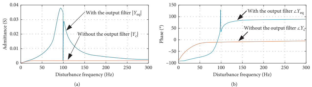
FIGURE 10: Characteristic of equivalent admittance (harmonic model) of the converter for the study case of Tables 1 and 2. (a) Magnitude of admittance. (b) Phase angle of admittance.
