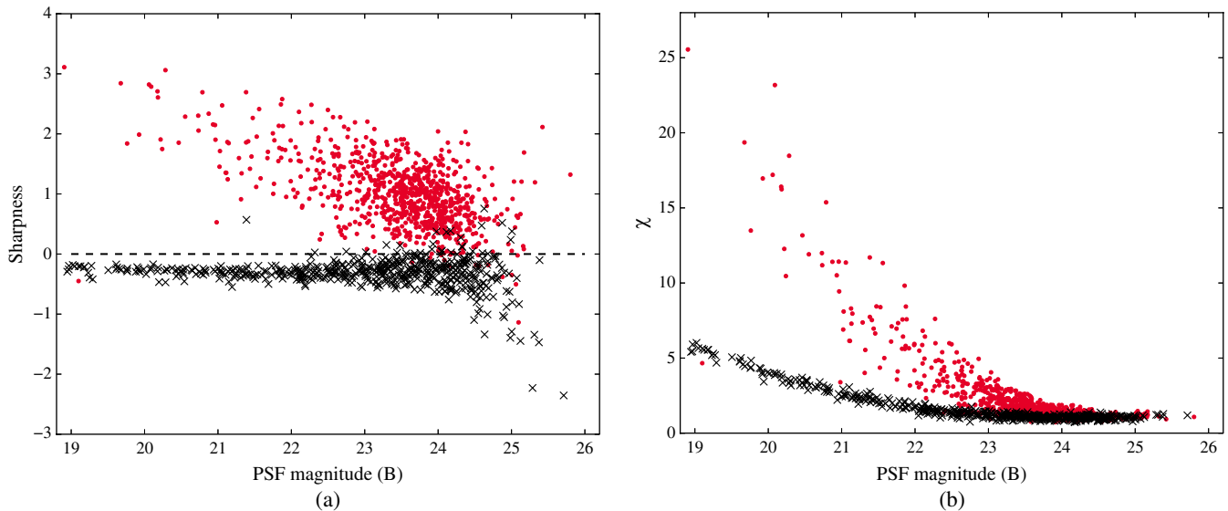
FIG. 4.—Distribution of DAOPHOT sharpness ( left panel ) and \chi ( right panel ) as a function of the PSF magnitude for simulated stars ( diagonal crosses ) and galaxies ( points ). In the left panel the dashed line at zero sharpness is the adopted separation limit for the star/galaxy classification (see § 5.2). See the online edition of the PASP for a color version of this figure.
