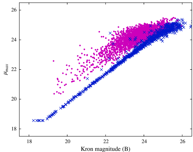
FIG. 1.— \mu_{\max} as a function of the Kron magnitude for stars ( diagonal crosses ) and galaxies ( points ) in the SExtractor catalog. See the online edition of the PASP for a color version of this figure.
