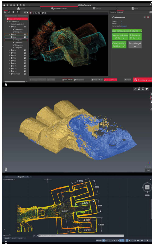
Fig. 9 – Tumulus 1, Sasso Pinzuto-Toscana: A) registration process between two cloud setups; B) 3D modeling separately from the cloud data; C) point cloud dimensioning at 1:1 scale.
