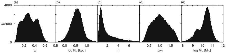
Fig. 19.2 Distribution of some galaxy parameters: photo- z , z (panel a ), r -band effective radius \log R_e/\text{kpc} (panel b ), r -band Sérsic index, n (panel c ), observer-frame g-r colour within an aperture of 3'' of radius (panel d ) and Chabrier IMF-based stellar mass \log M_*/M_\odot (panel e )
