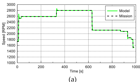
FIGURE 6. (a) Required speed mission in dashed line and calculated speed in green line; (b) Instantaneous ICE, EM, and Propeller power. These figures refer to the PH-268 (A) configuration.
