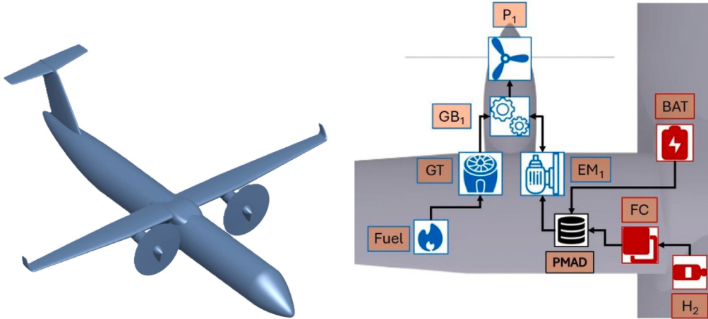
(a) Geometric 3D model of the 90-passenger hybrid-electric regional aircraft. (b) Assumed powerplant architecture of the 90-passenger hybrid-electric regional aircraft.
