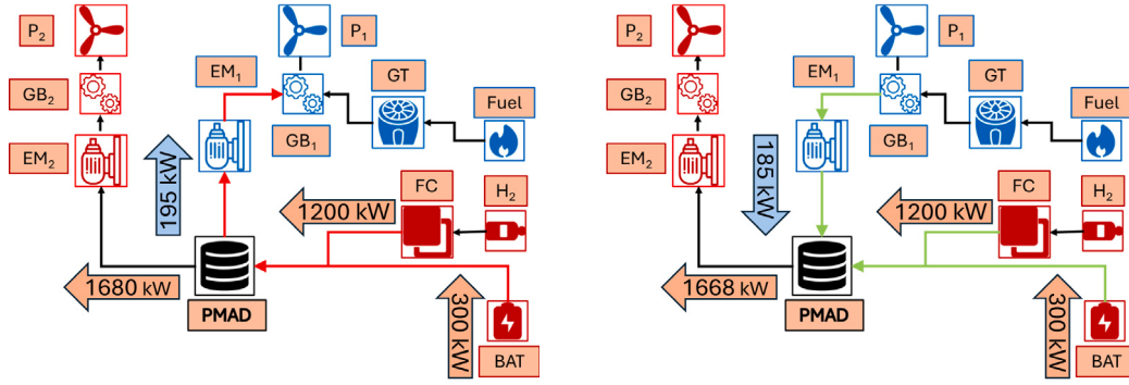
(a) Nonphysical power distribution for CASE ID 3-1, when EM_1 is forced to operate as a motor. This behavior produces an imbalance of power at the PMAD node.
