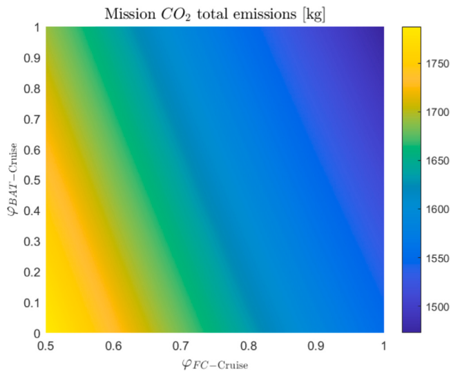
Fig. 12. Surface plot illustrating the total CO 2 emissions generated during the 300 nmi typical mission, presented as a function of the fuel cell ( \phi_{FC-Cruise} ) and battery ( \phi_{BAT-Cruise} ) throttle setting combinations selected for the cruise phase.
