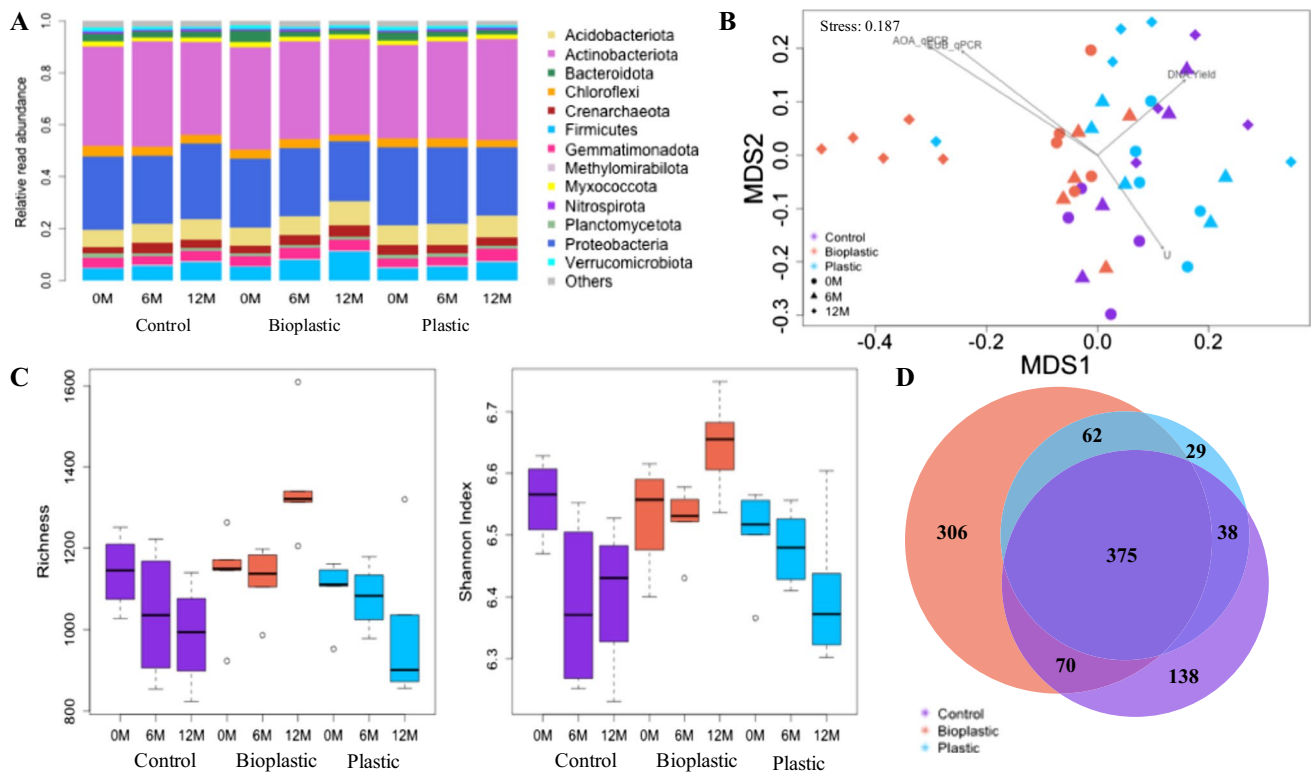
Fig. 3. Soil bacteriome overview exposed to different treatments (control: violet, bioplastic: coral, plastic: light blue) at the beginning (0M: circle), after six (6M: triangle) and twelve (12M: roar) months of the experiment. A Distribution of taxa across time course and soil samples. Amplicon sequence variants (ASVs) detected by Illumina Novaseq sequencing of the 16S V4 were summarized based on their phylum annotation. B Non-metric multidimensional scaling (NMDS)
