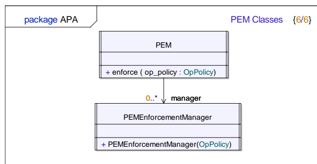
Fig. 8 Class Diagram of the PAM internal components
