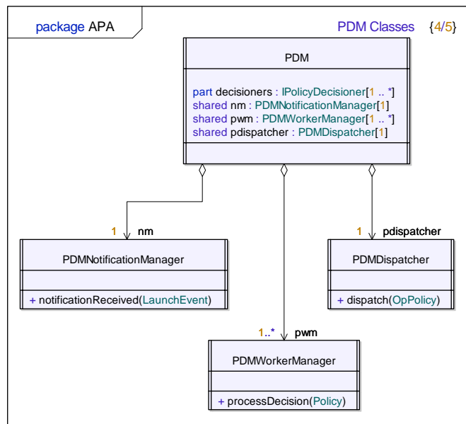
Fig. 4 Class Diagram of the PDM internal components
