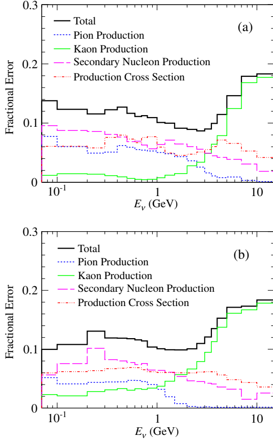
FIG. 7 (color online). The fractional hadron interaction errors on \nu_\mu (a), \nu_e (b) flux predictions at SK.
