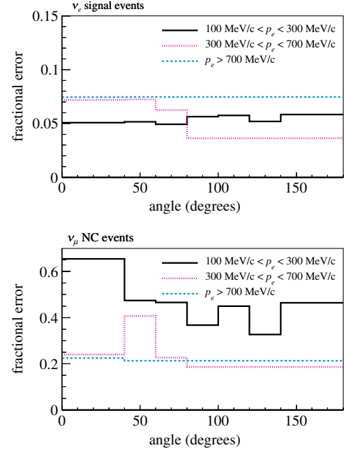
FIG. 29 (color online). The fractional errors on SK \nu_e signal (top) and NC background (bottom) predictions from the SK detector response uncertainty as a function of the electron candidate momentum and angle.
