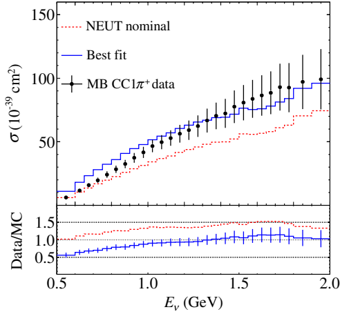
FIG. 13 (color online). The CC1 \pi^+ cross section as a function of energy as measured by MiniBooNE, with the NEUT nominal and best-fit models. The treatment in the analysis of the disagreement between the best-fit NEUT and data is discussed in the text.
