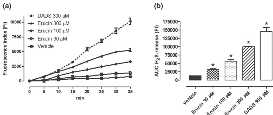
FIGURE 2 Fluorometric recording of erucin-mediated H 2 S-release inside HASMCs. (a) Time course of the fluorometric recordings of H 2 S released by vehicle, erucin 30, 100, and 300 \mu\text{M} and DADS 300 \mu\text{M} , during 35 min of observation: the increase in H 2 S is expressed as FI. (b) The histograms show the total amount of H 2 S released by vehicle, erucin 30, 100, and 300 \mu\text{M} and DADS 300 \mu\text{M} , in the 35 min of observation time, expressed as AUC. The vertical bars represent SEM, six different experiments were performed, each with six replicates ( n = 6 ). The asterisks indicate a statistically significant difference from vehicle ( *P < 0.05 )
