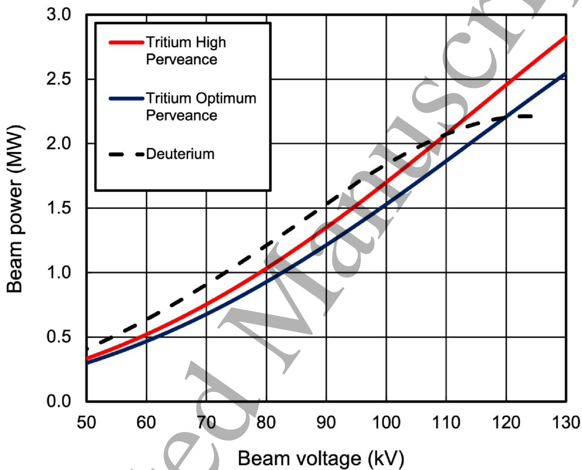
Figure 9: Neutral beam power of a JET Positive Ion Neutral Injector (PINI) when operated in deuterium (black dashed line) or tritium at either optimum perveance (blue full line) or increased perveance (red full line).
