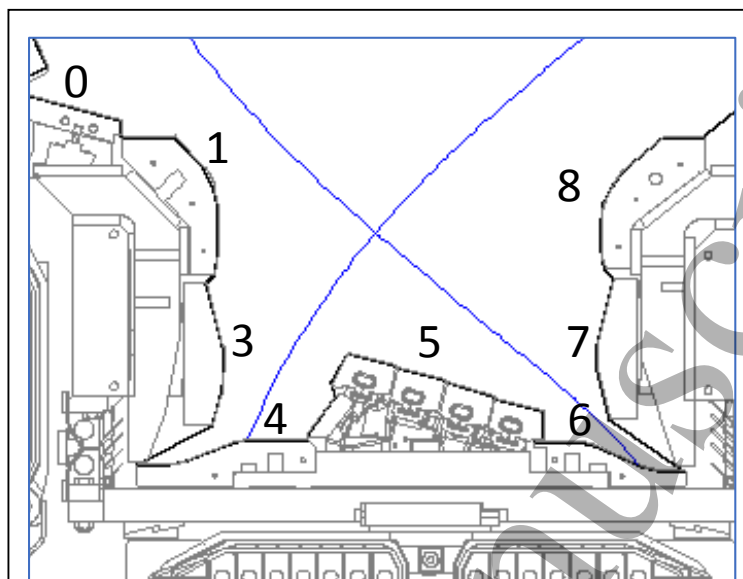
Figure 15 – JET-ILW divertor, with divertor tiles & location identified by numbers 0 to 8. The separatrix for a plasma configuration with inner and outer strike-points on tile 4 and 6 respectively is shown in blue. Tile 5 is composed of 4 ‘stacks’ identified as A to D from left to right.
