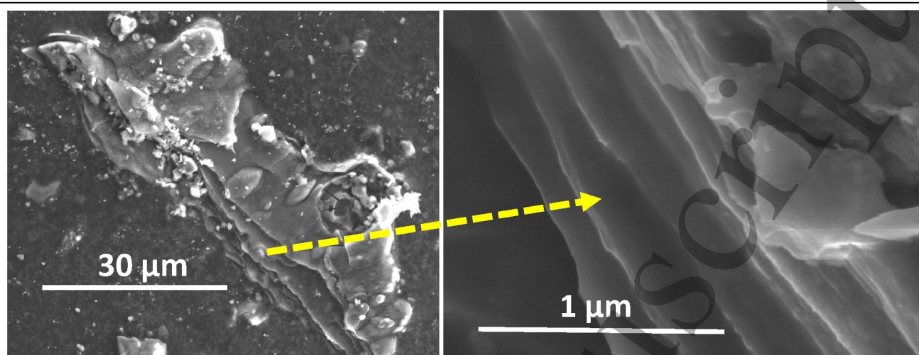
Figure 19. A flake of a stratified co-deposit containing mainly Be and C found on the Mascot wrist. Reproduced from [141].
