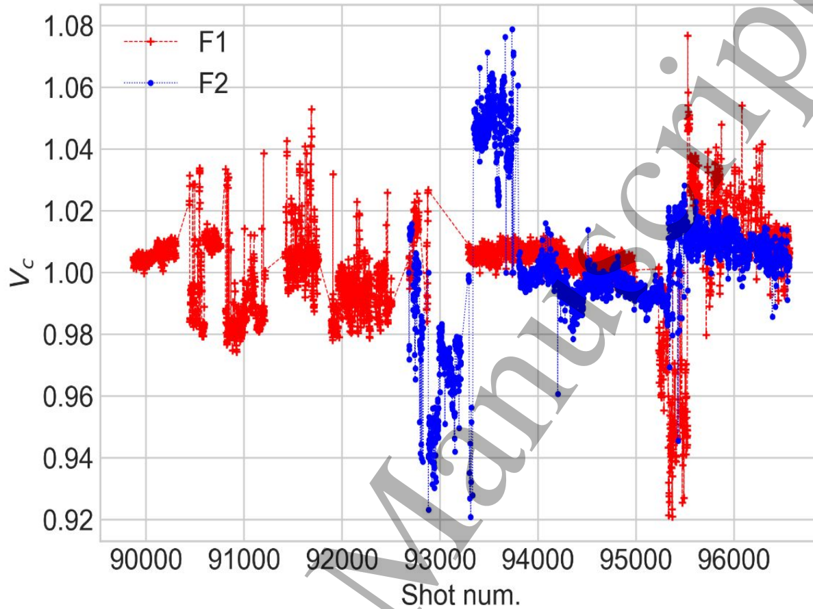
Figure 25. The normalised Verdet constant for FOCS 1 (F1, red) and FOCS 2 (F2, blue) systems during JET operation for shots from 89870 to 96563. The estimated values are 0.696 \pm 0.010 and 0.672 \pm 0.013 rad/MA, respectively.
