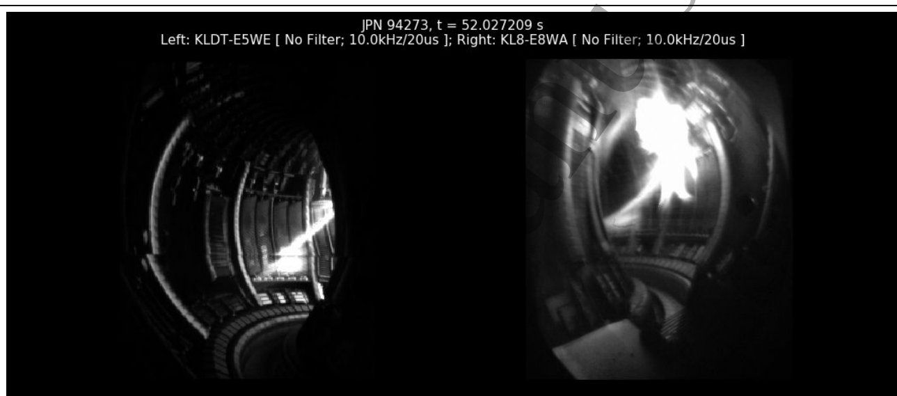
36 Figure 7 - D 2 SPI injection (from top right) in JET captured by highspeed visible light camera. 37 38 39 40 41 42 43 44 45 46 47 48 49 50 51 52 53 54 55 56 57 58 59 60
