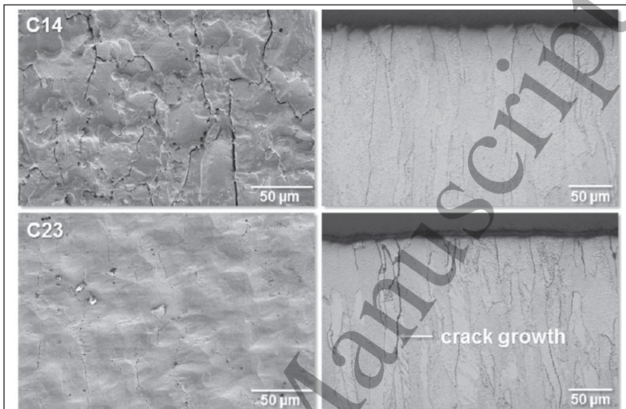
Figure 17. Microscopy images and metallographic cross sections of the lamellae C14 and C23. Reproduced from [146].
