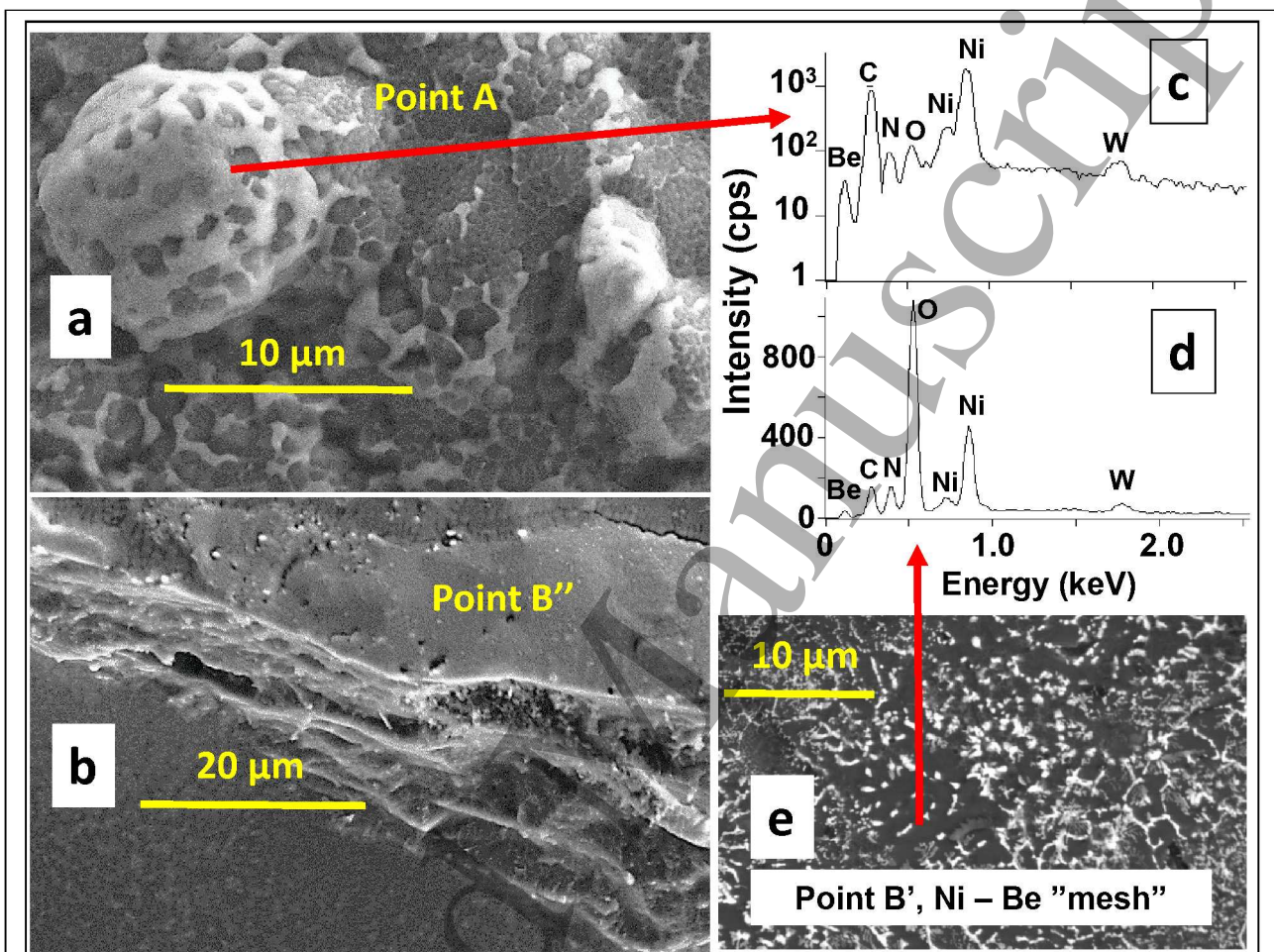
Figure 13. Surface structure and composition of co-deposits on the beryllium IWG limiter after all three ILW campaigns. Sampling areas A and B are marked in Figure 12. Fig. 13-e is reproduced from [174].
