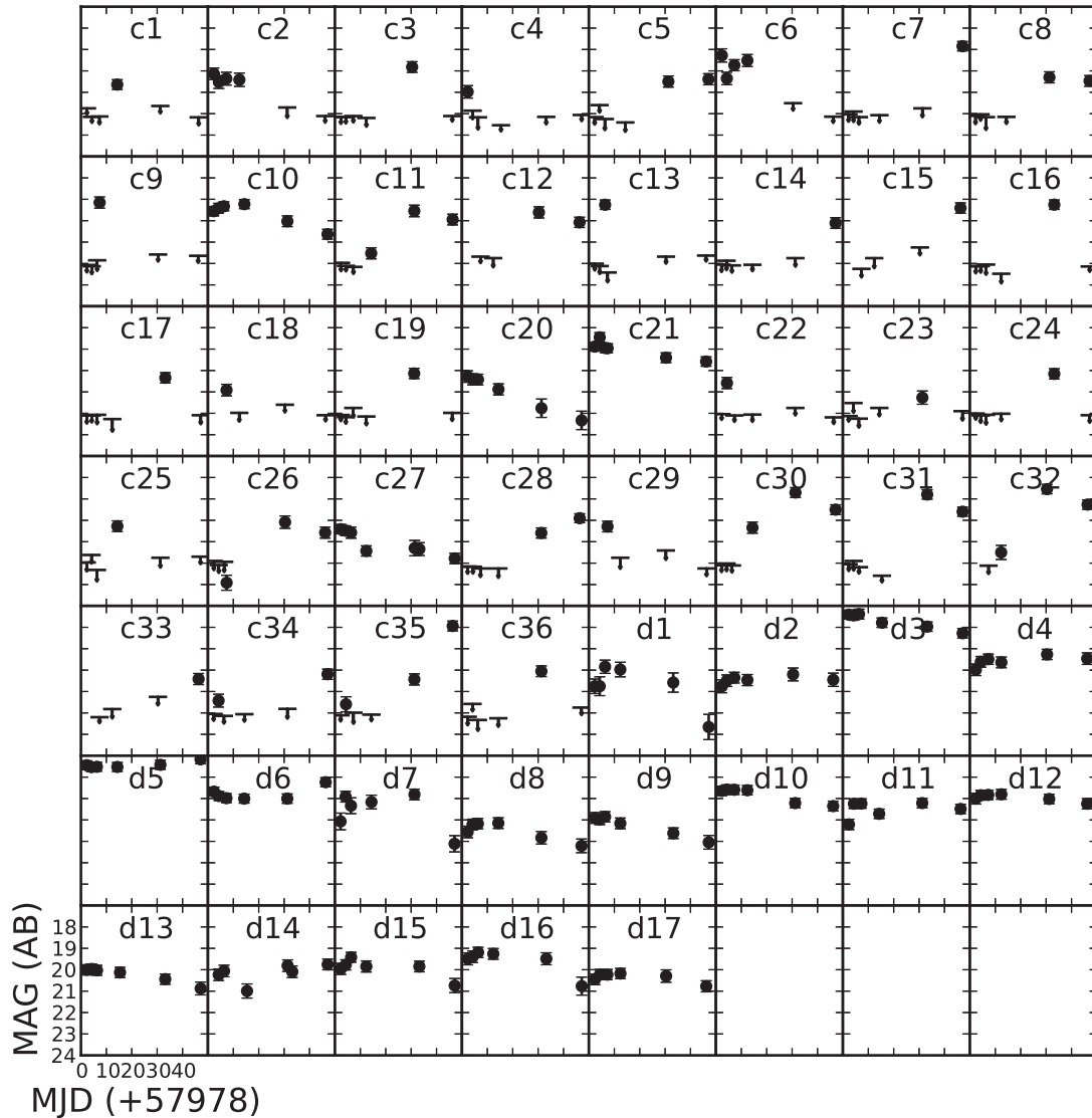
Figure 3. The light curves of the transient candidates found with the VST in 99 \text{ deg}^2 covering the GW170814 error area. Arrows indicate the upper limit magnitude for the undetected sources.
